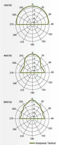
HORIZONTAL / VERTICAL POLAR DIAGRAMS
